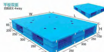
-1210PS-A(HJ) 带管 (with tube)
