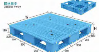
-1210WT-B(HJ) 带管 (with tube)
