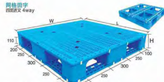
1210WT-B(HJ) 带管 (with tube)
