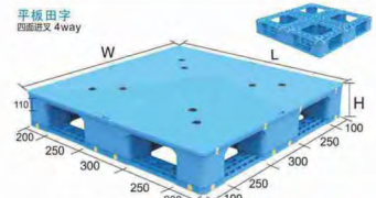
-1210PT-B(HJ) 带管 (with tube)
