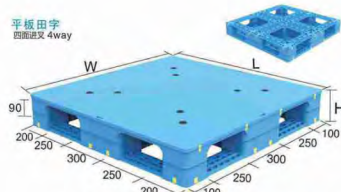
-1210PT-A(HJ) 带管 (with tube)
