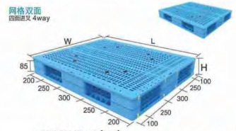
-1210WS-A(HJ) 带管 (with tube)
