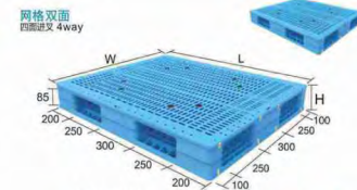
-1210WS-A(HJ) 带管 (with tube)
