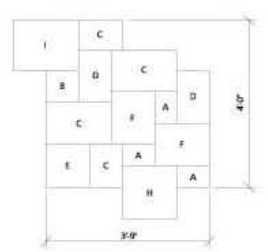
B82 Interlocking Unit Lays Out 4'-0" x 3'-9" or 15 Square Feet
