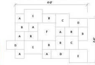
B80 Interlocking Unit Lays Out 4'-0" x 2'-6" or 10 Square Feet
