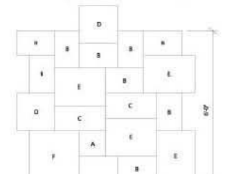
B84 Interlocking Unit Lays Out 6'-6" x 6'-0" or 39 Square Feet
