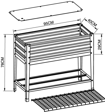
Item No. GM51080-S Size: 95 X 40 X 78CM (LX W X H) Depth: 29CM CTN QTY: 20'GP 670PCS/40' HQ: 1690PCS
