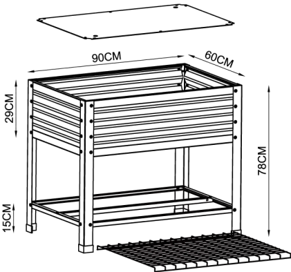
Item No. GM51080 Size: 90 X 60 X 78CM (LX W X H) Depth: 29CM CTN QTY: 20'GP 494PCS/40' HQ: 1244PCS
