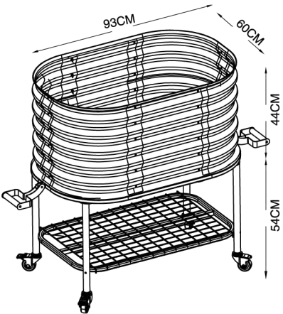
Item No. GM51081 Size: 93 X 60 X 98CM (LX W X H) Depth: 44CM CTN QTY: 20'GP 320PCS/40' HQ: 770PCS
