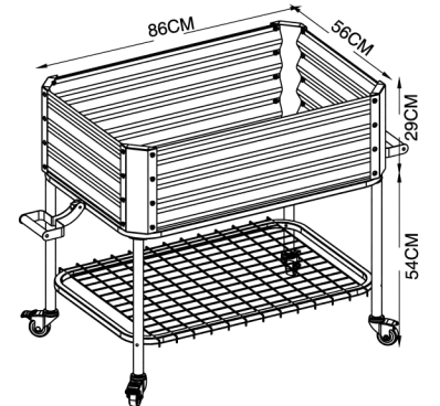
Item No. GM51082 Size: 86 X 56 X 84CM (LX W X H) Depth: 29CM CTN QTY: 20'GP 404PCS/40' HQ: 1018PCS
