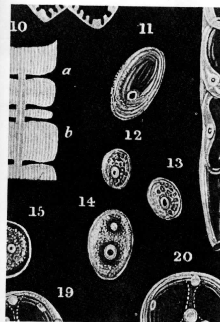
Fig. 6. Various cells drawn by Schleiden and Schwann (1847). Note that the nucleus and nucleolus were seen in most cells; 11 is a sporule from Rhizina laevigata , Fries; 12 – 14 are cytotlasts from the embryo sac of Pimelea drupacea ; 20 is a sporule of Marchantia polymorpha .
