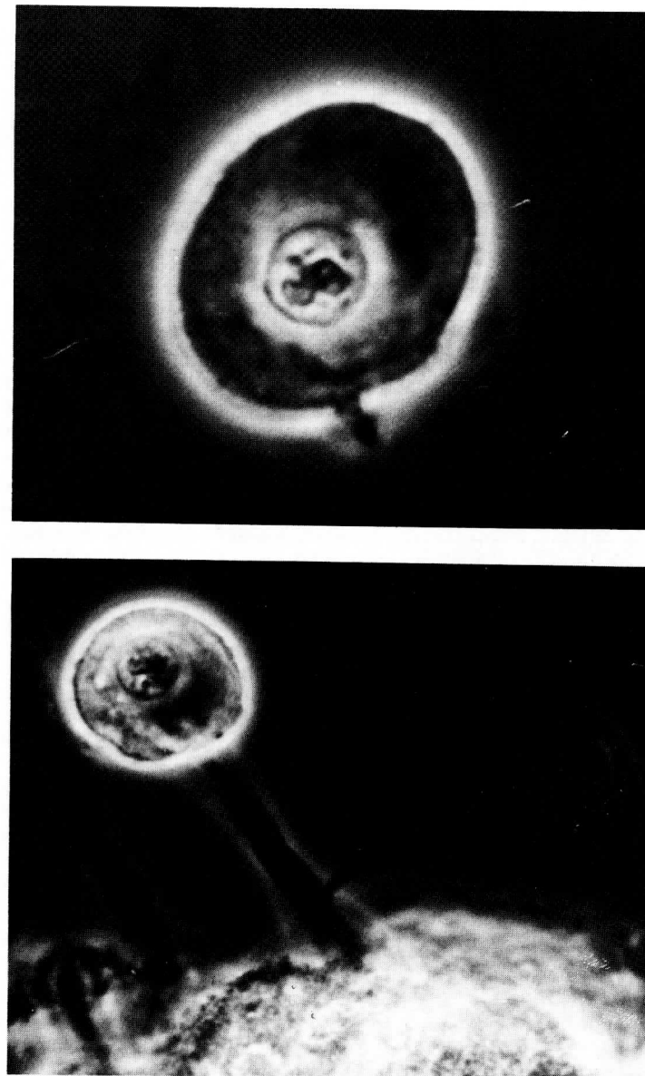
Fig. 18. Nuclei isolated in saline by hand dissection from rabbit medullary neurons; they are not fixed. The nuclei are 15–20 microns in diameter. Note the nucleolar membranes and the nucleolonema.
