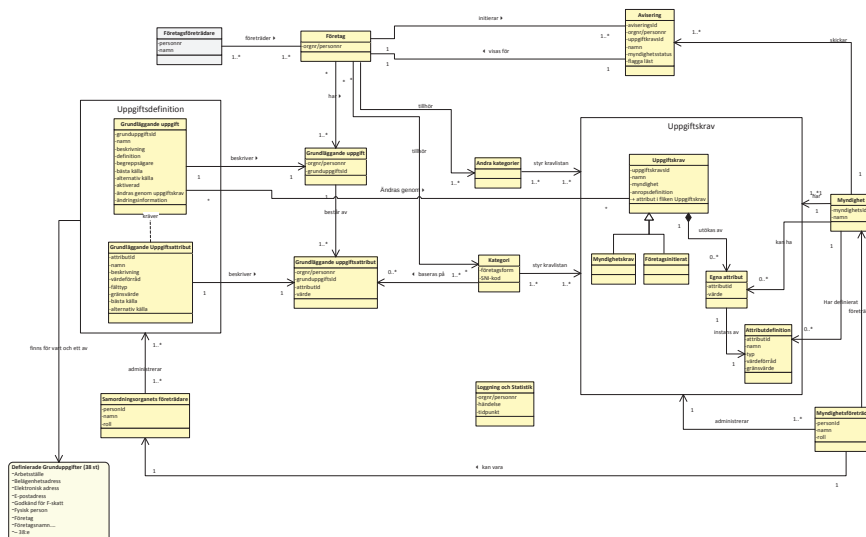
Figur 8 Informationsmodell
