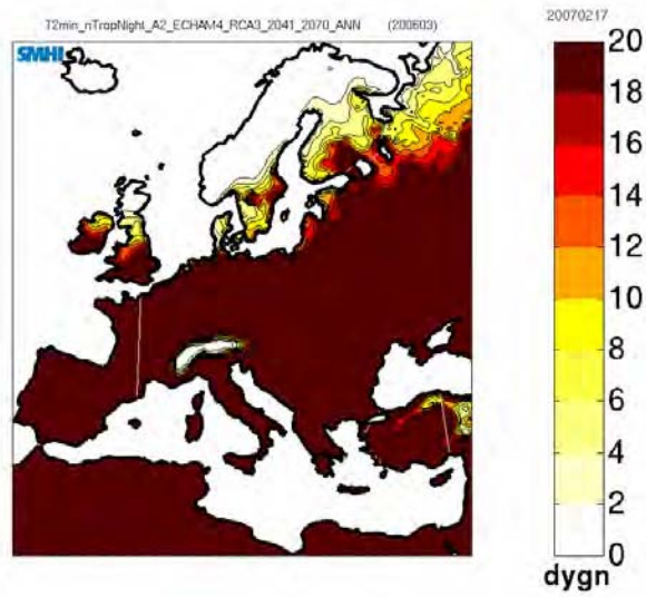
Figur 18 Antal tropiska nätter 2041–70 (Rossby Centre, SMHI, T2min_nTropNight_A2_ECHAM4_RCA3_2041_2070_ANN)
