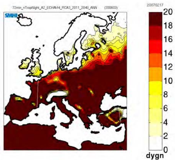
Figur 17 Antal tropiska nätter 2011–40 (Rossby Centre, SMHI, T2min_nTropNight_A2_ECHAM4_RCA3_2011_2040_ANN)
