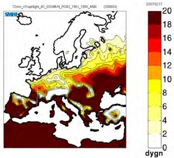
Figur 16 Antal tropiska nätter 1961–90 (Rossby Centre, SMHI, T2min_nTropNight_A2_ECHAM4_RCA3_1961_1990_ANN)
