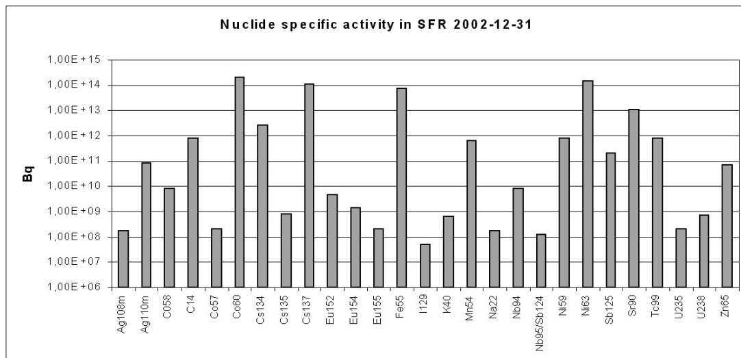
Figure D4: Nuclide specific inventory for most common isotopes in SFR-1.
