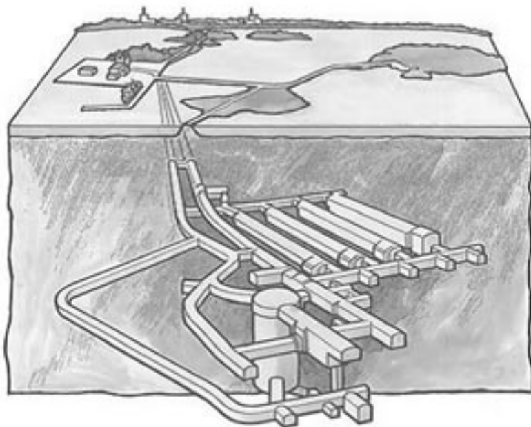
Figure D3: The repository for radioactive operational waste (SFR)
