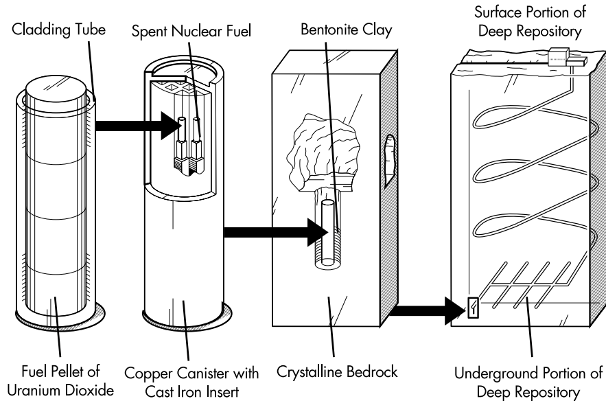
Figure A6: The KBS-3 method is SKB's reference method for disposal of spent nuclear fuel.
