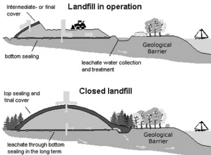
Figure D5: Principle section of a shallow land burial at OKG.
