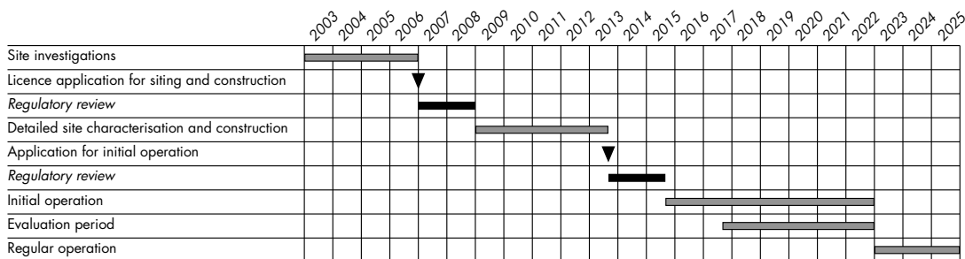
Figure A3: Time schedule for disposal of the spent nuclear fuel.
