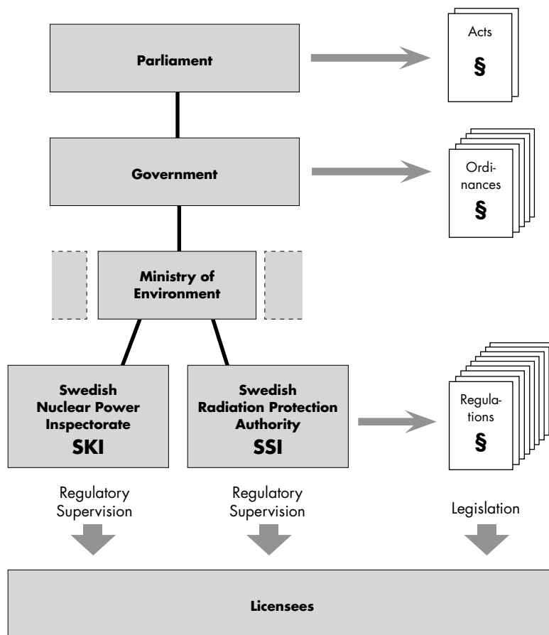
Figure A5: Organisational structure for nuclear safety and radiation protection supervision.
