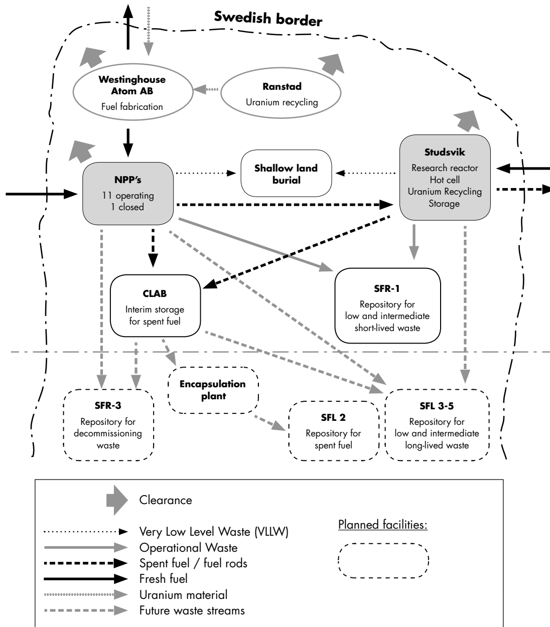
Figure A4: Material and waste streams in the Swedish nuclear fuel cycle.
