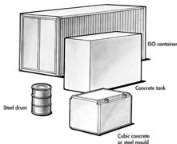
Figure D2: Standard packages for short-lived LILW used in Sweden.
