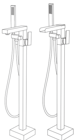
Assembly Drawing
