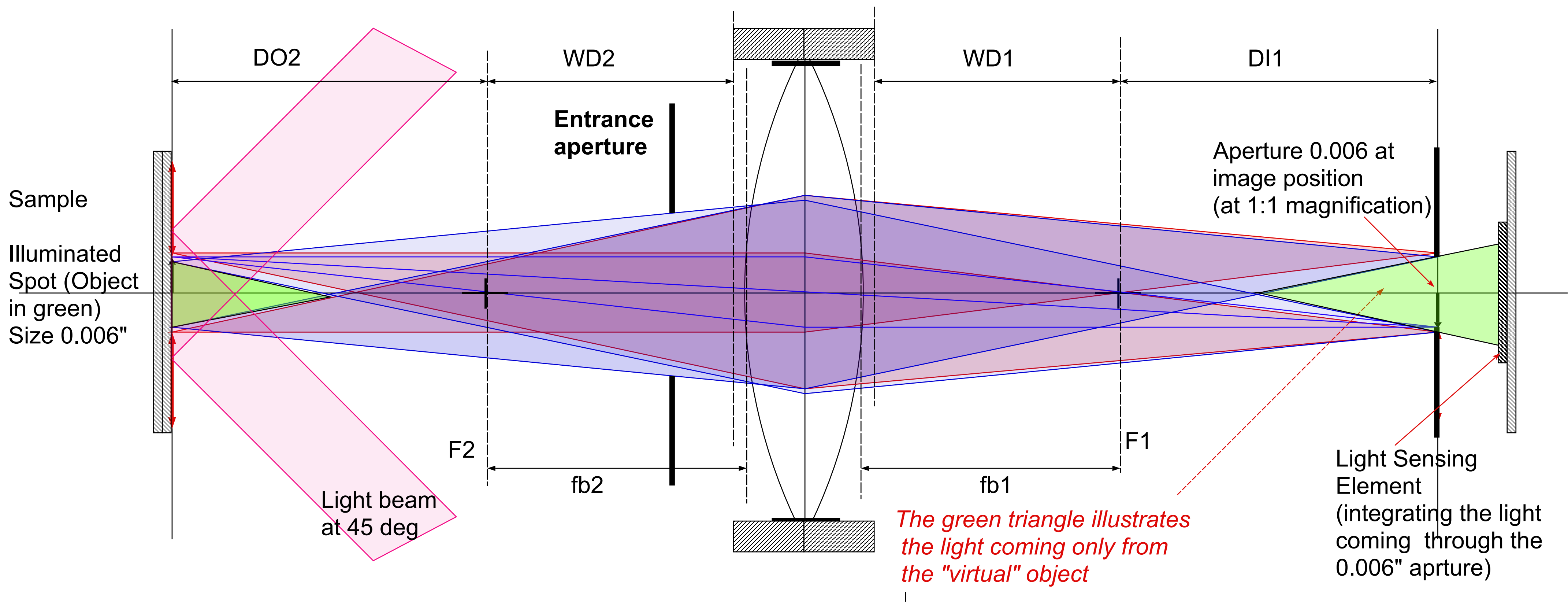
Reference Optical Arrangement (with ray tracing)
