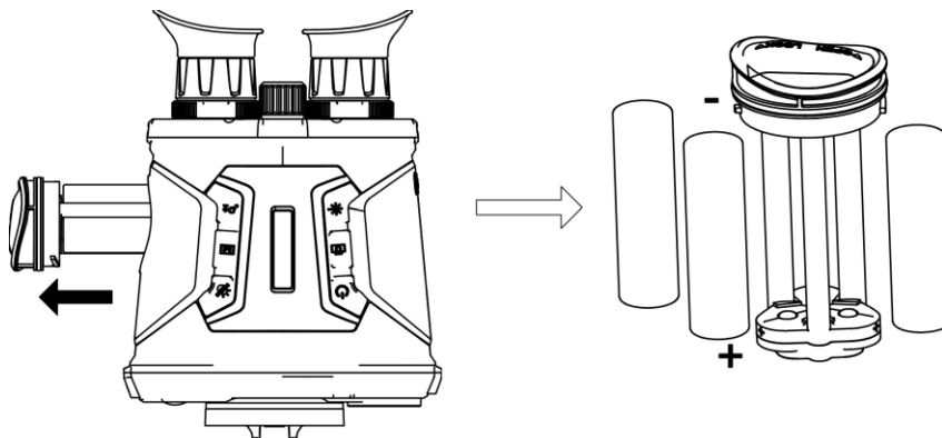
Figure 2-3 Install Batteries
