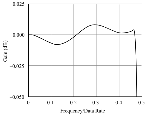
Figure 6. Typical Passband Response for the NI-9234
