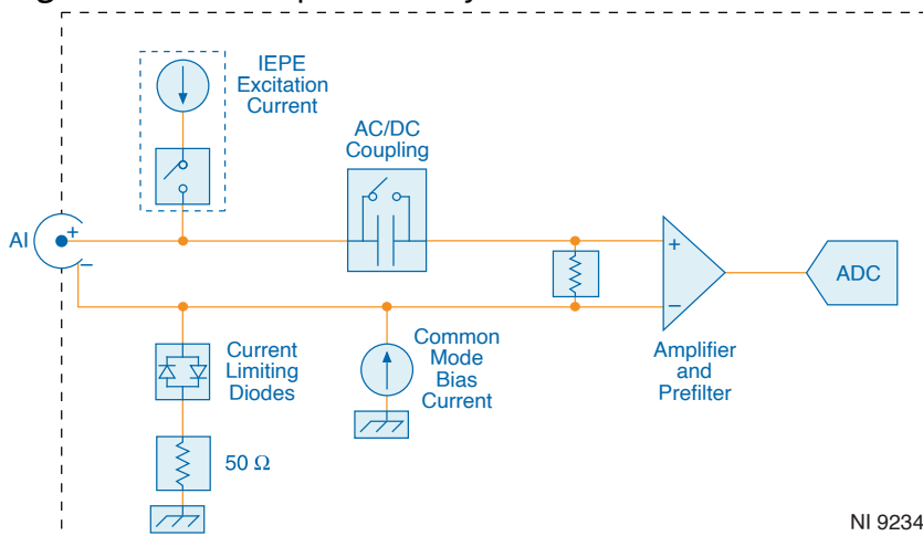
Figure 5. NI-9234 Input Circuitry for One Channel
