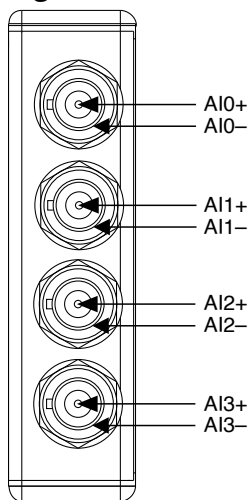
Figure 1. NI-9234 Pinout
